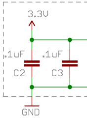
32u4 BYPASS
